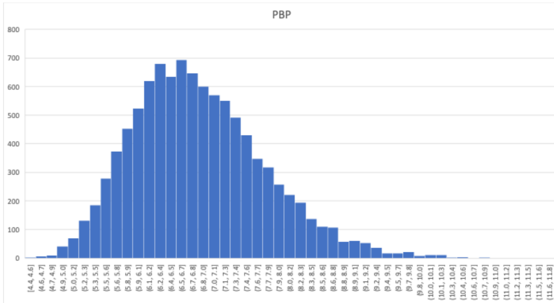
Fig 7: Probability distribution graph for PBP
