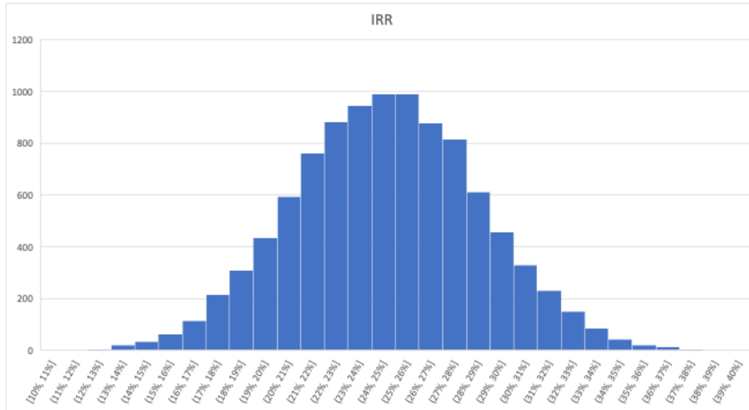
Fig 5: Probability distribution graph for the IRR
