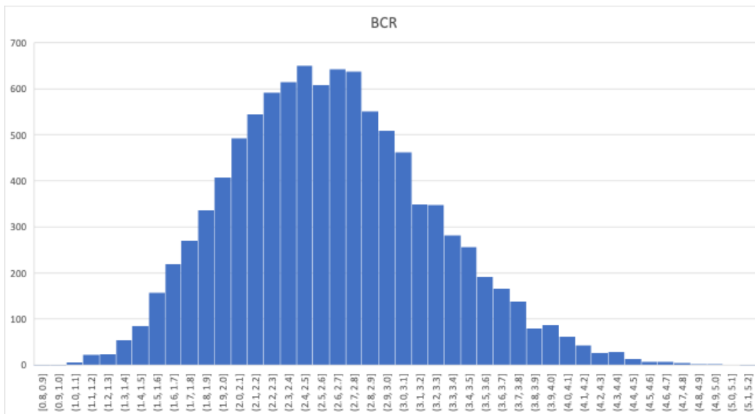
Fig 8: Probability distribution graph for the BCR
