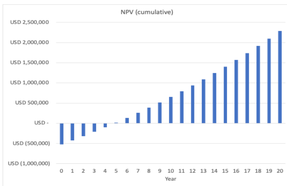
Fig 4: Accumulated cash flow (cumulative NPV)
