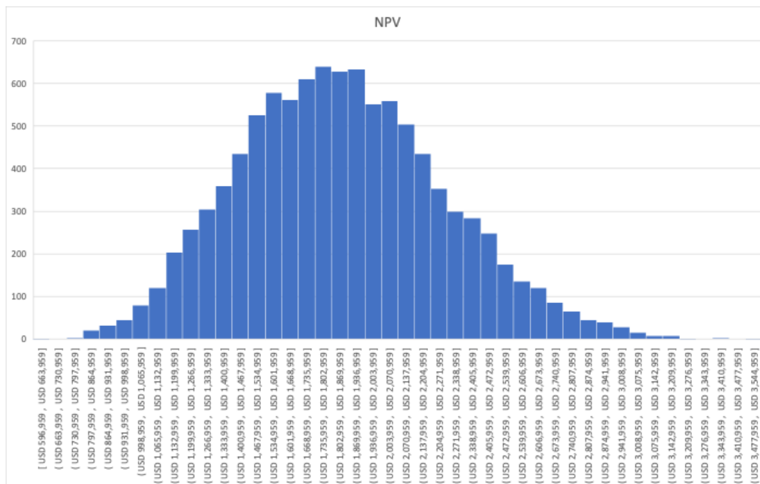
Fig 6: Probability distribution graph for NPV
